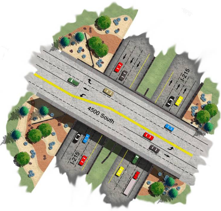
Site Plan
